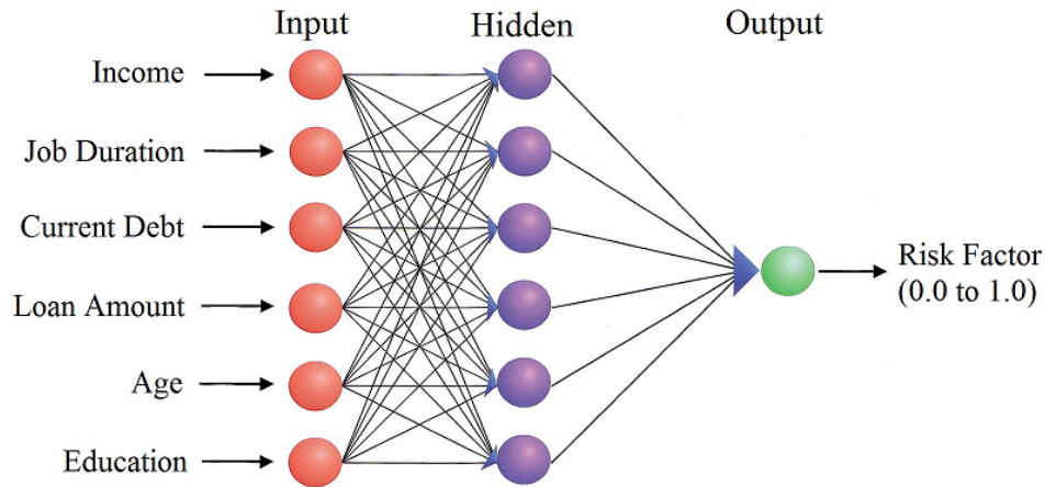
Figure 4: Machine Learning
