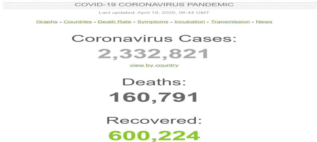
Figure 18: COVID-19 result
