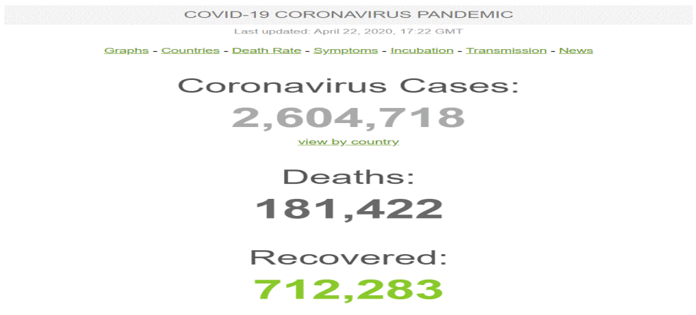
Figure 17: COVID-19 status
