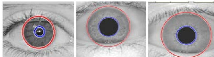
Figure 4: Boundary detections
